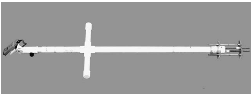
Figure 3. Handheld field probe (Bad Boy III) developed by the USDA/ARS/SWCRU for rapid in-field analysis of soil electrical conductivity (overall length 150 cm).
