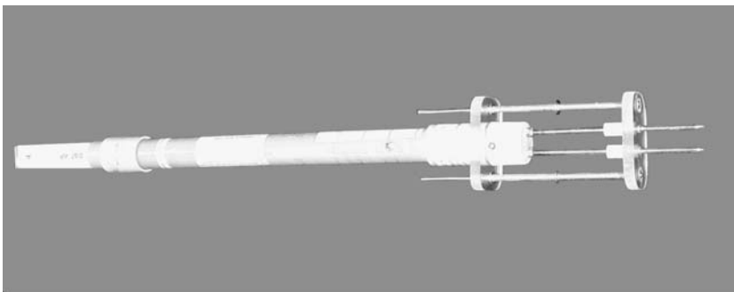
Figure 2. Handheld field probe (Bad Boy II) developed by the USDA/ARS/SWCRU for rapid in-field calibration and analysis of soil electrical conductivity (overall length 75 cm).
